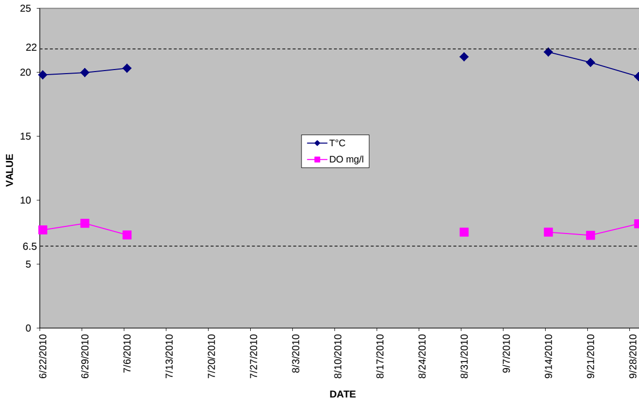
Figure 25. Daily average temperature (T) and rolling monthly average dissolved oxygen (DO) at GIP4, Gulf Island Pond, at dates and from depths where T \leq 22^{\circ}\text{C} to the bottom of the first meter of the thermocline or penultimate depth, 2010
