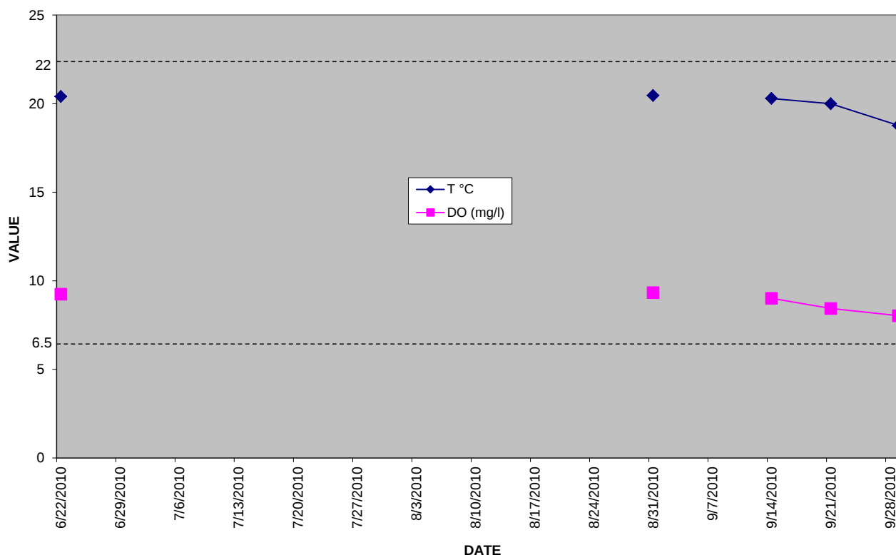
Figure 23. Daily average temperature (T) and rolling monthly average dissolved oxygen (DO) at Upper Narrows (UN), Gulf Island Pond, at dates and from depths where T \leq 22^{\circ}\text{C} to the penultimate depth, 2010
